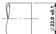
Tube Detail
